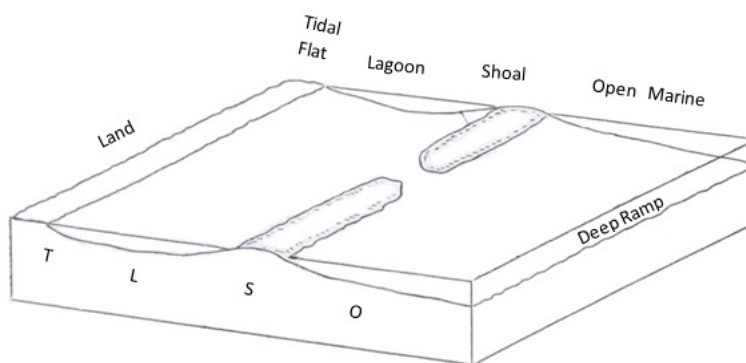
T: Tidal flat facies L: Lagoonal facies S: Shoal facies O: Open marin facies
